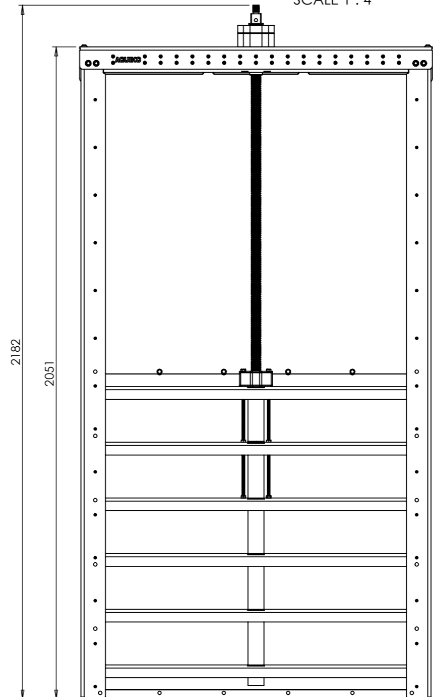
DETAIL A SCALE 1 : 4
